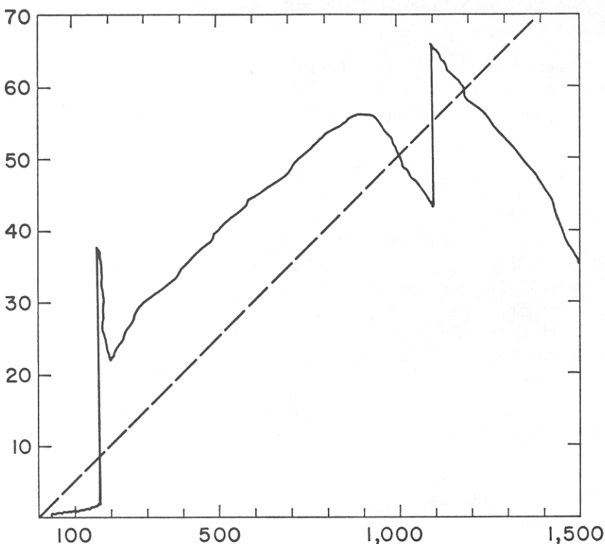
FIGURE C15-3. Sequential variation of the sample kurtosis of the daily changes of \log Z(t) , where Z(t) is the spot price of cotton, 1900-1905. The abscissa is the sample size. Linear coordinates.
