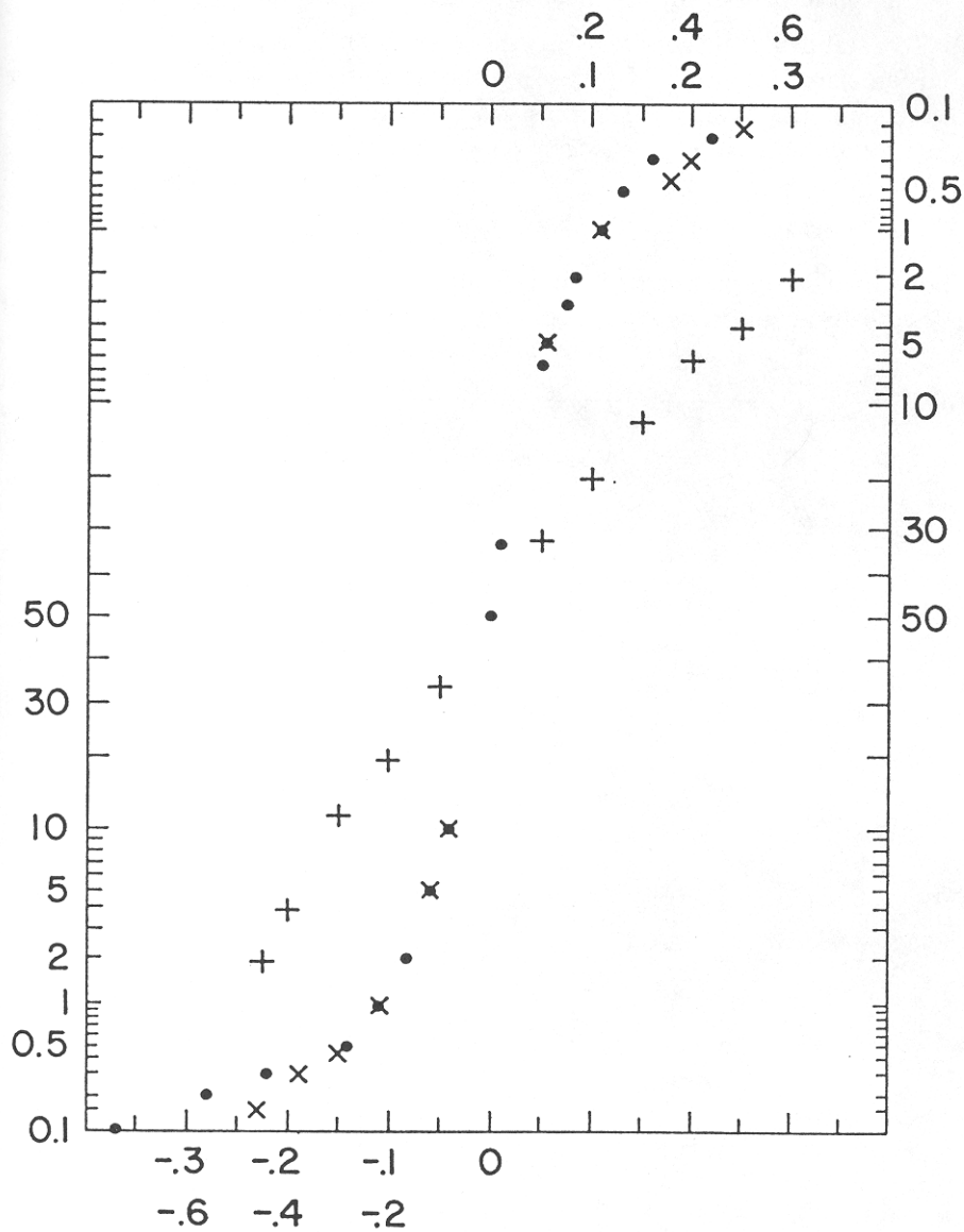
FIGURE C15-4. Probability-paper plots of the distribution of changes of \log Z(t) , where Z(t) is the spot price of wheat in Chicago, 1883-1934, as reported by Working 1934. The scale -0.3, -0.2, -0.1, 0, 0.1, 0.2, 0.3 applies to the weekly changes, marked by dots, and to the yearly changes, marked by crosses. The other scale applies to changes over lunar months, marked by \times .
