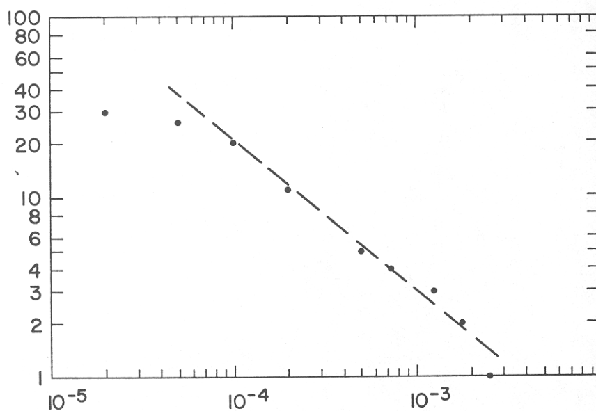
FIGURE C15-2. Cumulated absolute-frequency distribution for the data of Figure 1. Abscissa: log of the sample second moment. Ordinate: log of the absolute number of instances where the sample moment marked as abscissa has been exceeded. The L-stable model predicts a straight line of slope \alpha/2 \sim 1.7/2 , which is plotted as a dashed line.
