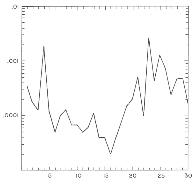
FIGURE C15-1. Sample second moment of the daily change of \log Z(t) , where Z(t) is the spot price of cotton. The period 1900-1905 was divided into thirty successive fifty-day samples, and the abscissa designates the number of the sample in chronological order. Logarithmic ordinate. A line joins the sample points to improve legibility.
