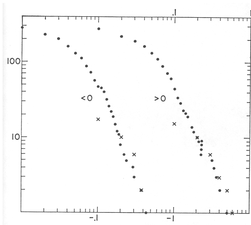
FIGURE C15-5. Weekly changes of \log Z(t) , where Z(t) is the price of wheat as reported by Working 1934. Ordinate: log of the absolute frequency with which L \geq u , respectively L \leq -u . Abscissas: the lower scale refers to negative changes, the upper scale to positive changes.
